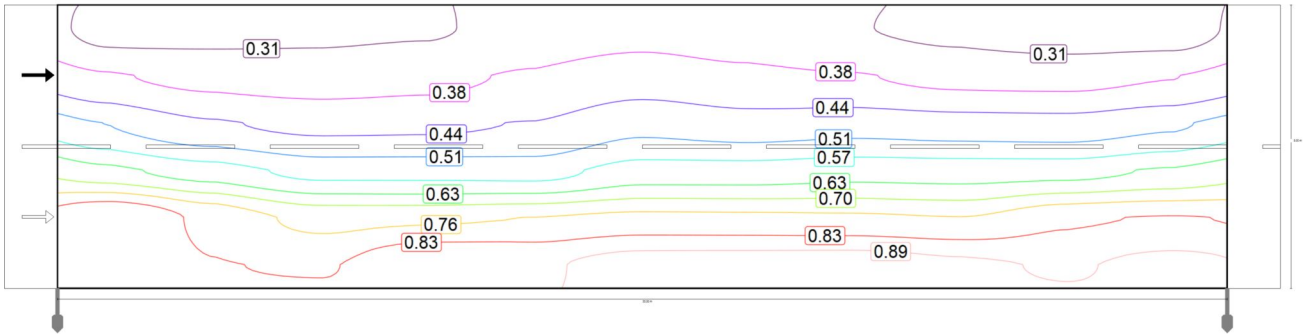
Observer 2: Maintenance value, luminance with dry roadway [cd/m²] (Iso-illuminance curves)
