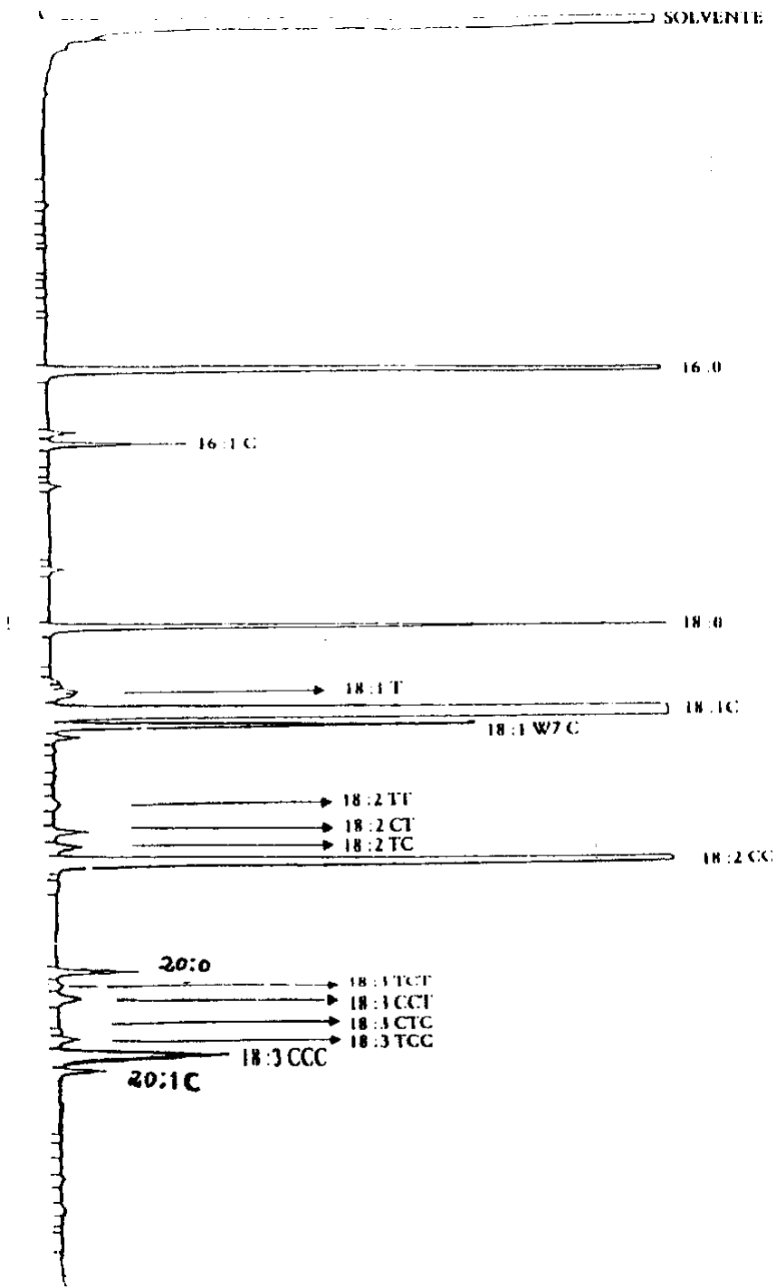
Figure 3: Specimen chromatogram obtained from by capillary column analysis of the trans fatty acids.
