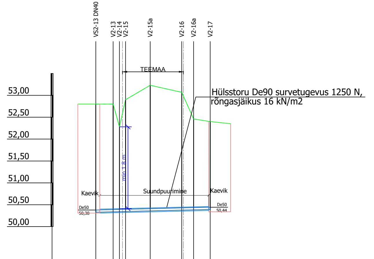
Pikiprofil 2 13129 km 7.10
