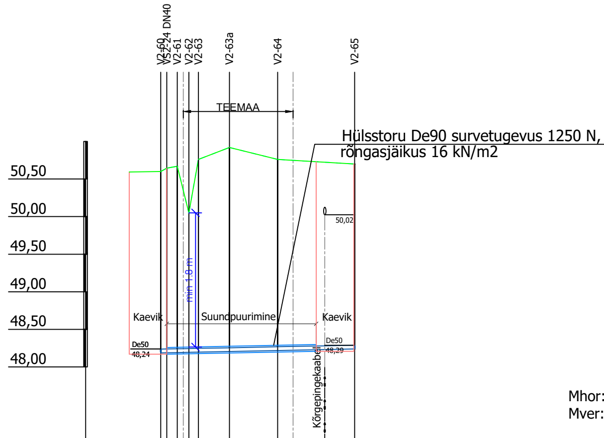
Pikiprofil 1 13129 km 6.480
