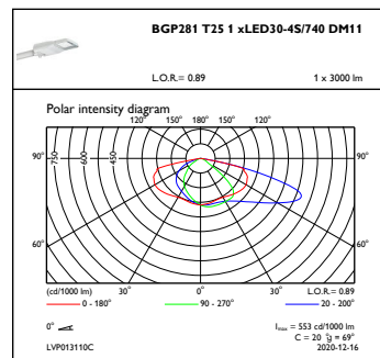
OFPC1_BGP281T251xLED30-4S740DM11
