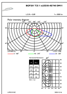
OFPL1_BGP281T251xLED30-4S740DM11
