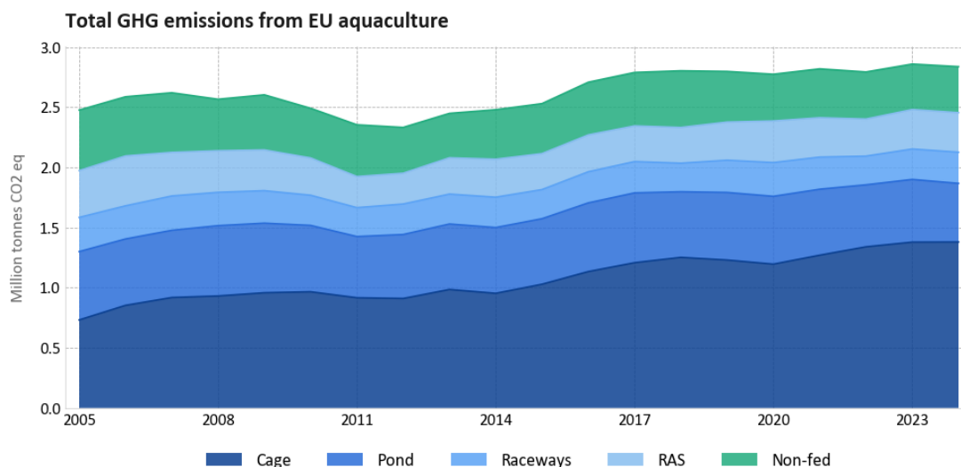
Figure 1 Trends in GHG emissions from the EU aquaculture sector by production system
