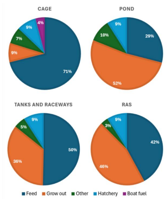
Figure 4 Contribution to fed aquaculture emissions in EU Member States of different processes and stages during the last 20 years for specific production systems. Source: EU Aquaculture: Greenhouse Gas Reduction Costs and Pathways to Net Zero by 2050 (2025)
