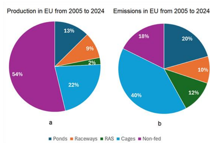
Figure 3 Aquaculture production (a) and associated emissions (b) from different production methods in EU from 2005 to 2024. Source: EU Aquaculture: Greenhouse Gas Reduction Costs and Pathways to Net Zero by 2050 (2025)
