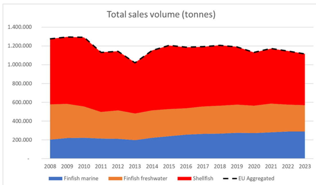
Figure 2 Trends in production volume from the EU aquaculture sector by production system
