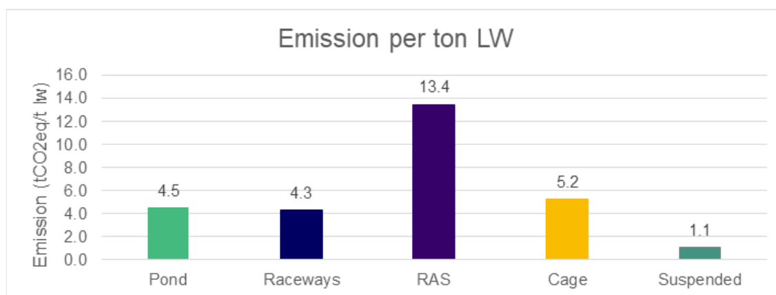
Figure 5 Total emission forecast per tonne of LW, 2026-2050 across production systems
