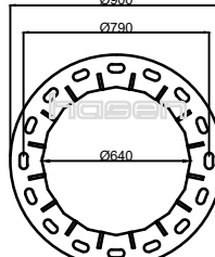
TABAN PLAKASI (hsn Base plate)
