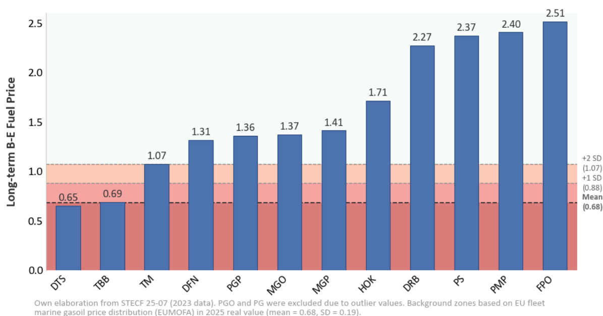
Figure 4 – Long-term break-even fuel price by fishing technique, and mean and distribution of EU marine gas oil (MGO) price
