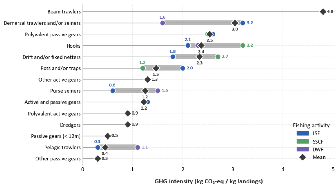
Figure 2 – CO 2 -equivalent emissions per kilogram of landings by fishing technique
